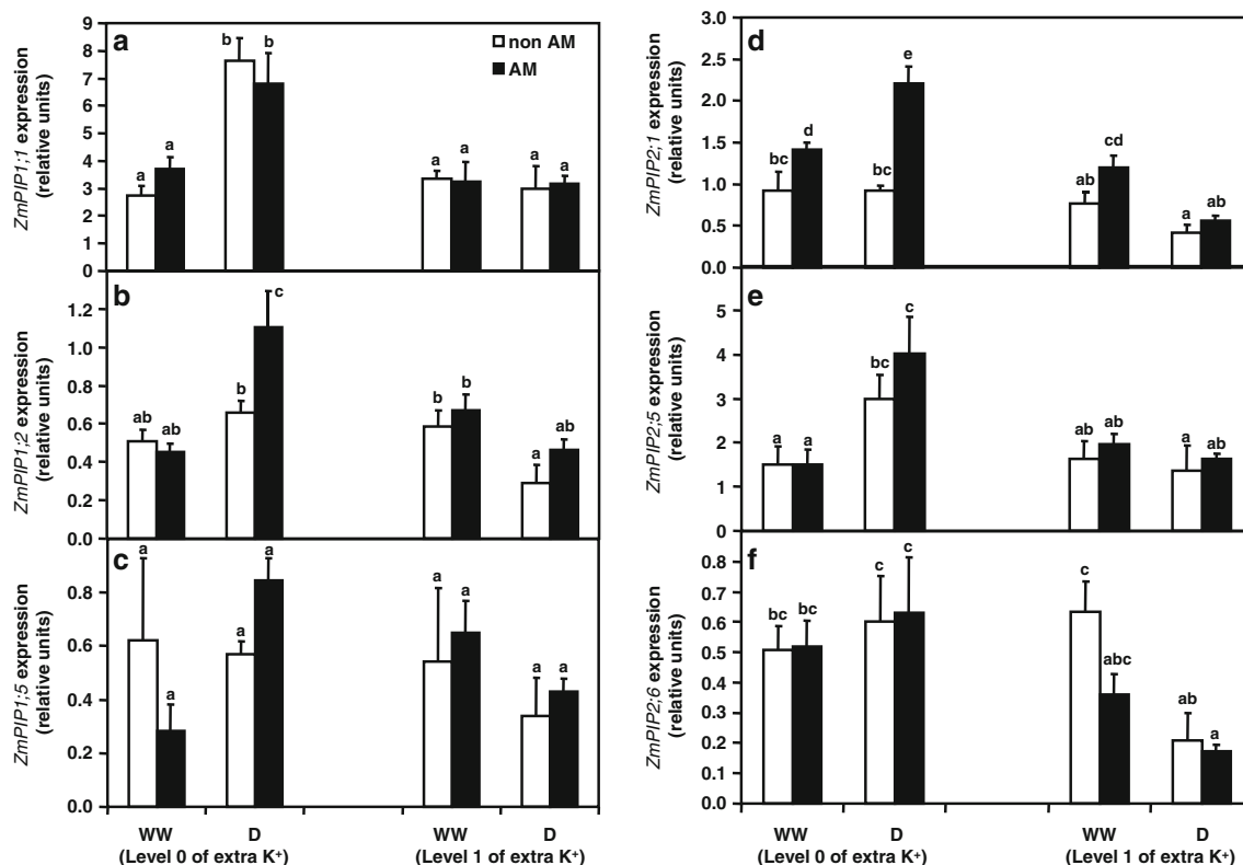
Fig. 4 Root expression of ZmPIP1;1 (a), ZmPIP1;2 (b), ZmPIP1;5 (c), ZmPIP2;1 (d), ZmPIP2;5 (e) and ZmPIP2;6 genes of AM (black bars) or non-AM (white bars) maize plants, grown well-watered (WW) or subjected to drought (D) under conditions of no extra potassium
