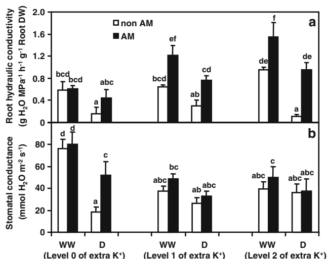
Fig. 2 Root hydraulic conductivity (a) and stomatal conductance (b) of AM (black bars) or non-AM (white bars) maize plants, grown well-watered (WW) or subjected to drought (D) under conditions of no extra potassium added, or levels 1 and 2 of extra K^+ . Bars represent mean \pm SE ( n=5 ). Different letters indicate significant differences among treatments ( p<0.05 ) after ANOVA and LSD tests
