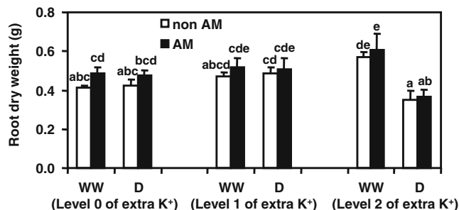
Fig. 1 Root dry weight of AM (black bars) or non-AM (white bars) maize plants, grown well-watered (WW) or subjected to drought (D) under conditions of no extra potassium added, or levels 1 and 2 of extra K^+ . Bars represent mean \pm SE ( n=5 ). Different letters indicate significant differences among treatments ( p<0.05 ) after ANOVA and LSD tests
